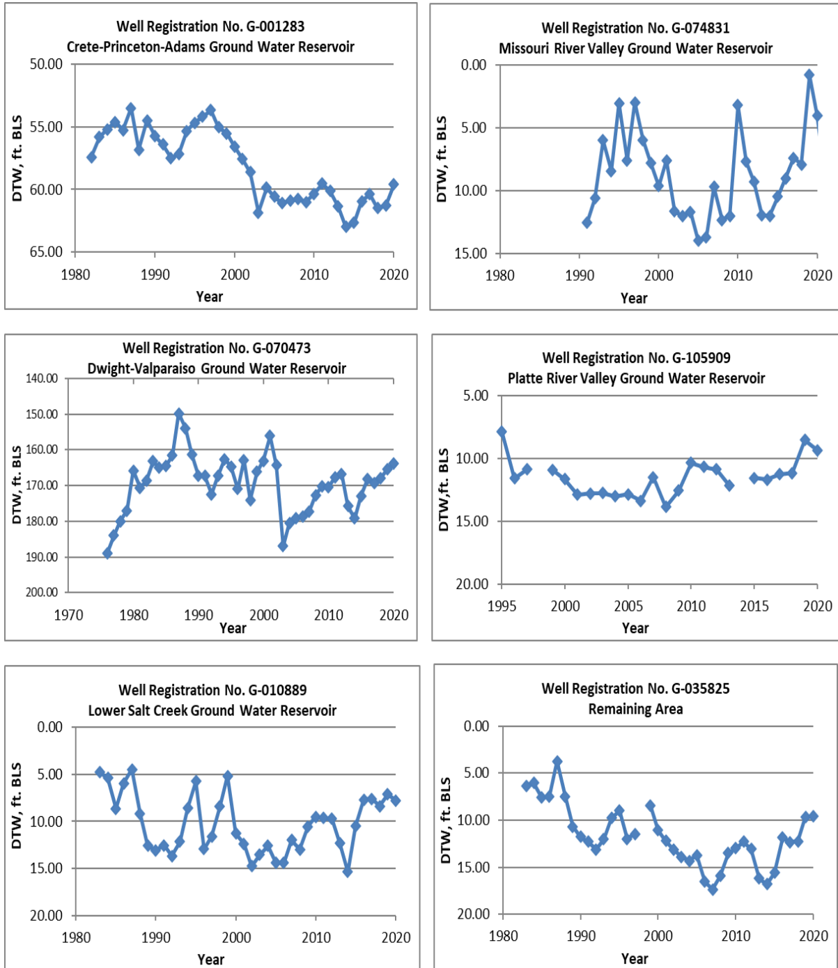
Figure 11 – Representative Spring Groundwater Level Graphs from Each Groundwater Reservoir
