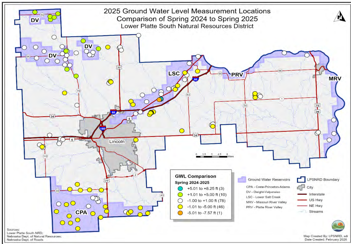
Figure 9: 2025 Groundwater level measurement comparison, spring 2024 and spring 2025.
